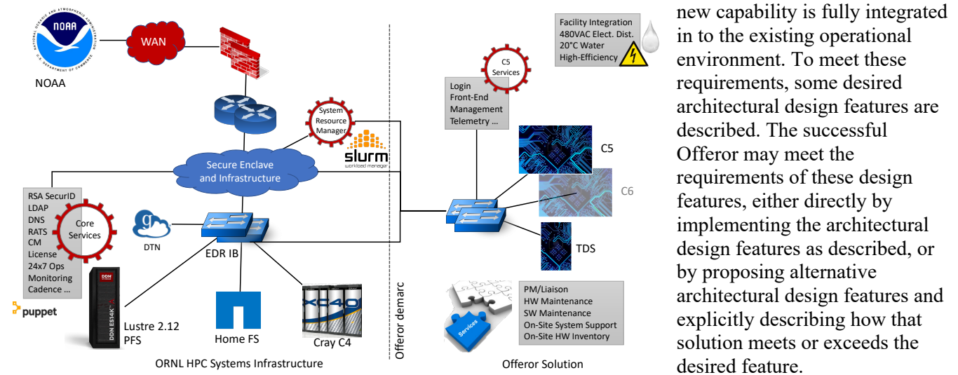
Figure 3-1. Notional C5 Design
